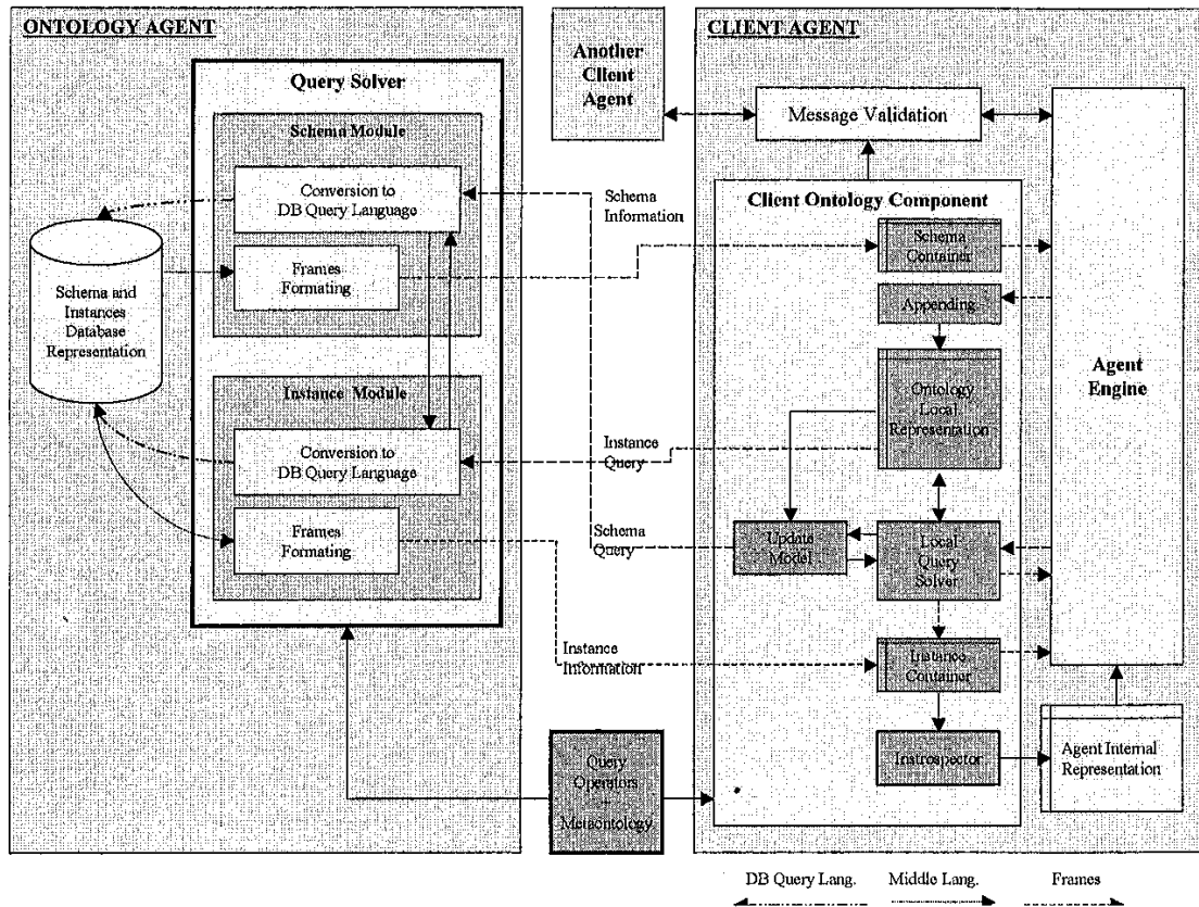
Fig. 2. Ontology handling architecture
