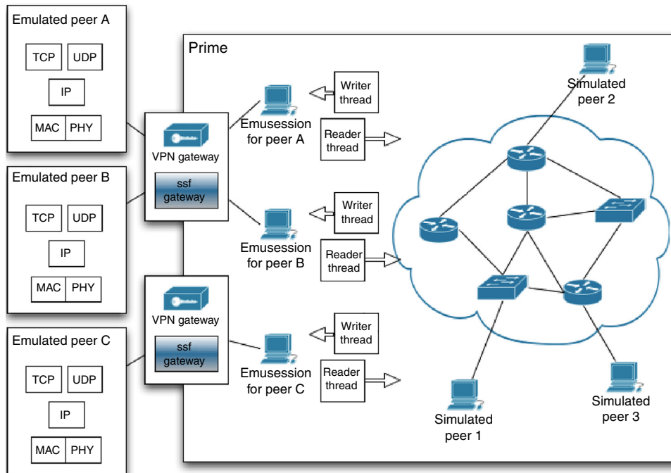
Fig. 2. Bit-SiEm structure.
