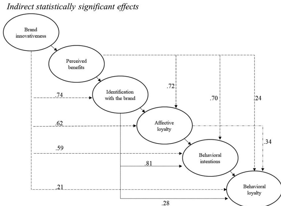
Figure 3. Indirect statistically significant effects.
